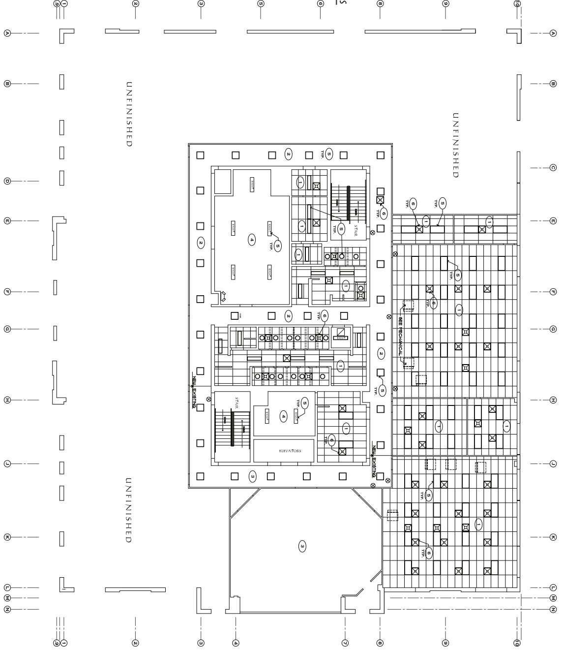
1 THIRD FLOOR REFLECTED CEILING PLAN SCALE: 1/8" = 1'-0"
